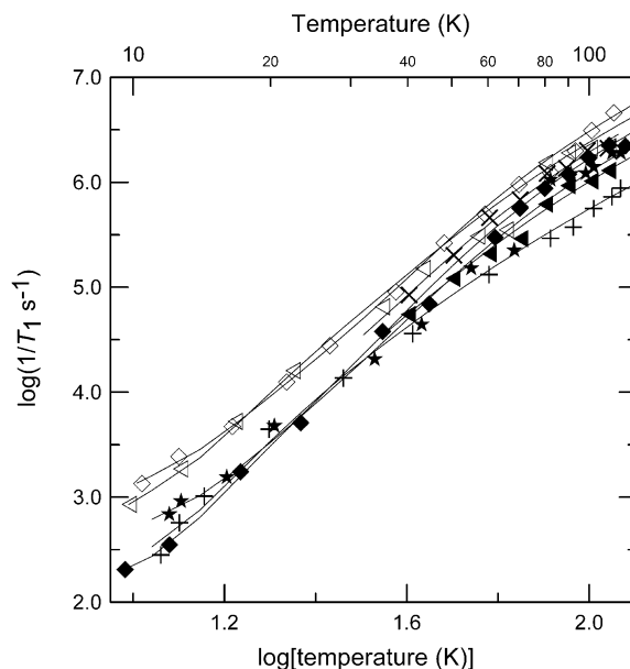
Fig. 6. Temperature dependence of X-band spin–lattice relaxation rates for the perpendicular lines in the spectra of 1 (+), 8 (◇) in 2:1 toluene/chloroform; Cu-S100A12 (◊), Cu/Ca-S100B (◆) and Cu-S100B (×) in buffer/glycerol; prion peptide HGGGW (★), and prion protein (23–28, 57–91) (◀) in buffer/glycerol. The solid lines through the data are fits obtained using Eq. (2) and the parameters in Table 2.
