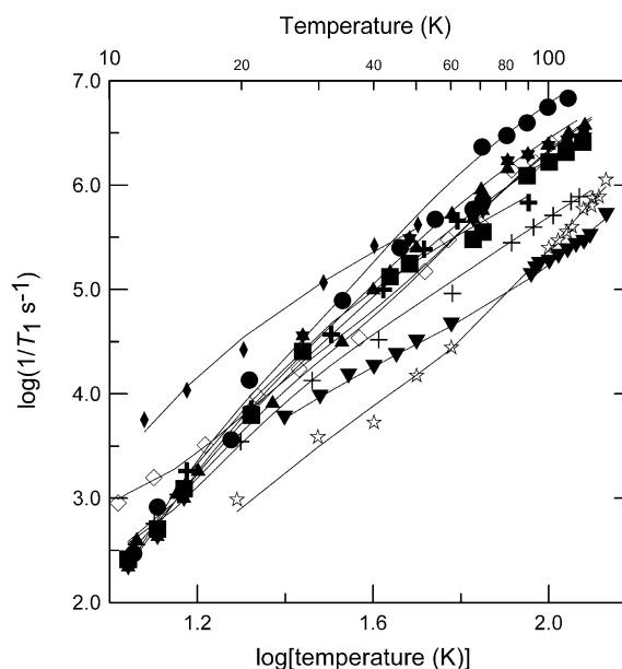
Fig. 10. Temperature dependence of X-band spin-lattice spin relaxation rates for the perpendicular lines in the spectra of 1 (+), 8 ( \diamond ), \text{Cu}(\text{dtc})_2 ( \blacktriangledown ), \text{CuTTP} ( \star ), \text{ZnTTPbipy-Cu}(\text{hfac})_2 ( \blacklozenge ), and \text{Cu}(\text{hfac})_2(\text{Me}_2\text{-bipy}) ( \blacklozenge ) in 2:1 toluene/chloroform solution; \text{CuEDTA} ( \star ), and \text{Cu}(\text{aq})^{2+} ( \bullet ) in water/glycerol (1:1); \text{Cu}(\text{OH})_4^{2-} in 3 M NaOH solution ( \blacksquare ); \text{CuIm}_4 ( \blacktriangle ) in 1:1 water/ethylene glycol. T_1 values were calculated using a single exponent fit to the data. The solid lines through the data are fits obtained using Eq. (2).
