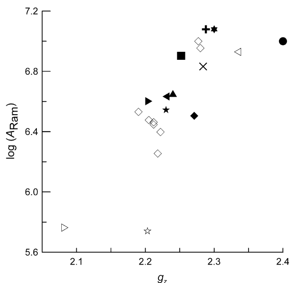
Fig. 11. Dependence of \log(A_{\text{Ram}}) on g_z for pyrrolate–imine copper(II) complexes 1–8 in 2:1 toluene/chloroform solution (◊); Cu-S100A12 (◁), Cu/Ca-S100B (◆), and Cu-S100B (×) in buffer/glycerol; prion peptide HGGGW (★) and prion protein (23–28, 57–91) (◀) in buffer/glycerol; CuEDTA (★), and Cu(aq) 2+ (●) in 1:1 water/glycerol; Cu(OH) 4 2- (■) in 3 M NaOH solution; CuIm 4 (▲) and CuMeIm 4 (▶) in 1:1 water/ethylene glycol; Cu(dtc) 2 in Ni(dtc) 2 (▷), CuTTP (☆), ZnTTPbipy-Cu(hfac) 2 (⊕) in 2:1 toluene/chloroform.
