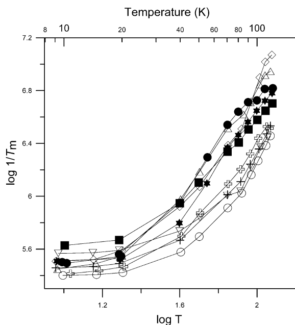
Fig. 7. Temperature dependence of X-band spin-spin relaxation rates for the perpendicular lines in the spectra of 1 (+), 2 (⊕), 3 (▽), 4 (○), 7 (△), and 8 (◇) in 2:1 toluene/chloroform solution; CuEDTA (★), and Cu(aq) 2+ (●) in water/glycerol (1:1); and Cu(OH) 4 2- in 3 M NaOH solution (■). T_m obtained using a fixed exponent of one. The lines connect the data points.
