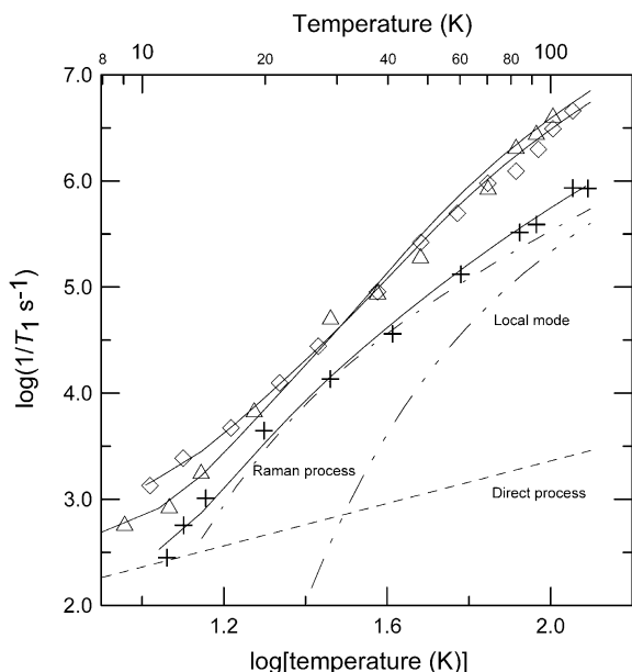
Fig. 3. Temperature dependence of X-band spin–lattice relaxation rates for the perpendicular lines in the spectra of 1 (+), 7 ( \Delta ), and 8 ( \diamond ) in 2:1 toluene/chloroform solution. The solid lines through the data are fits obtained using Eq. (2) and the parameters in Table 2. The contributions to the relaxation for 1 from the direct process (---), Raman process (----) and local mode (-----) are shown separately.
